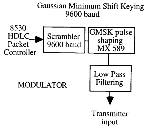
Figure 5: Modem Modulator
