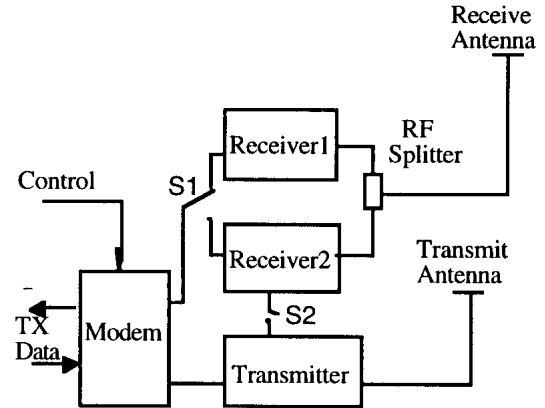
Figure 2: Flight Segment
