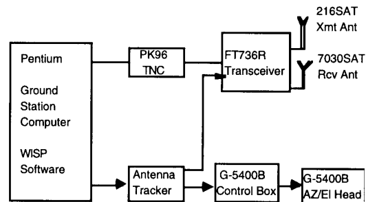
Figure 7: Ground Station
