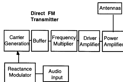
Figure 4: Transmitter
