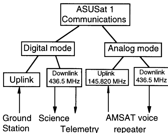
Figure 1: ASUSat 1 Communications
